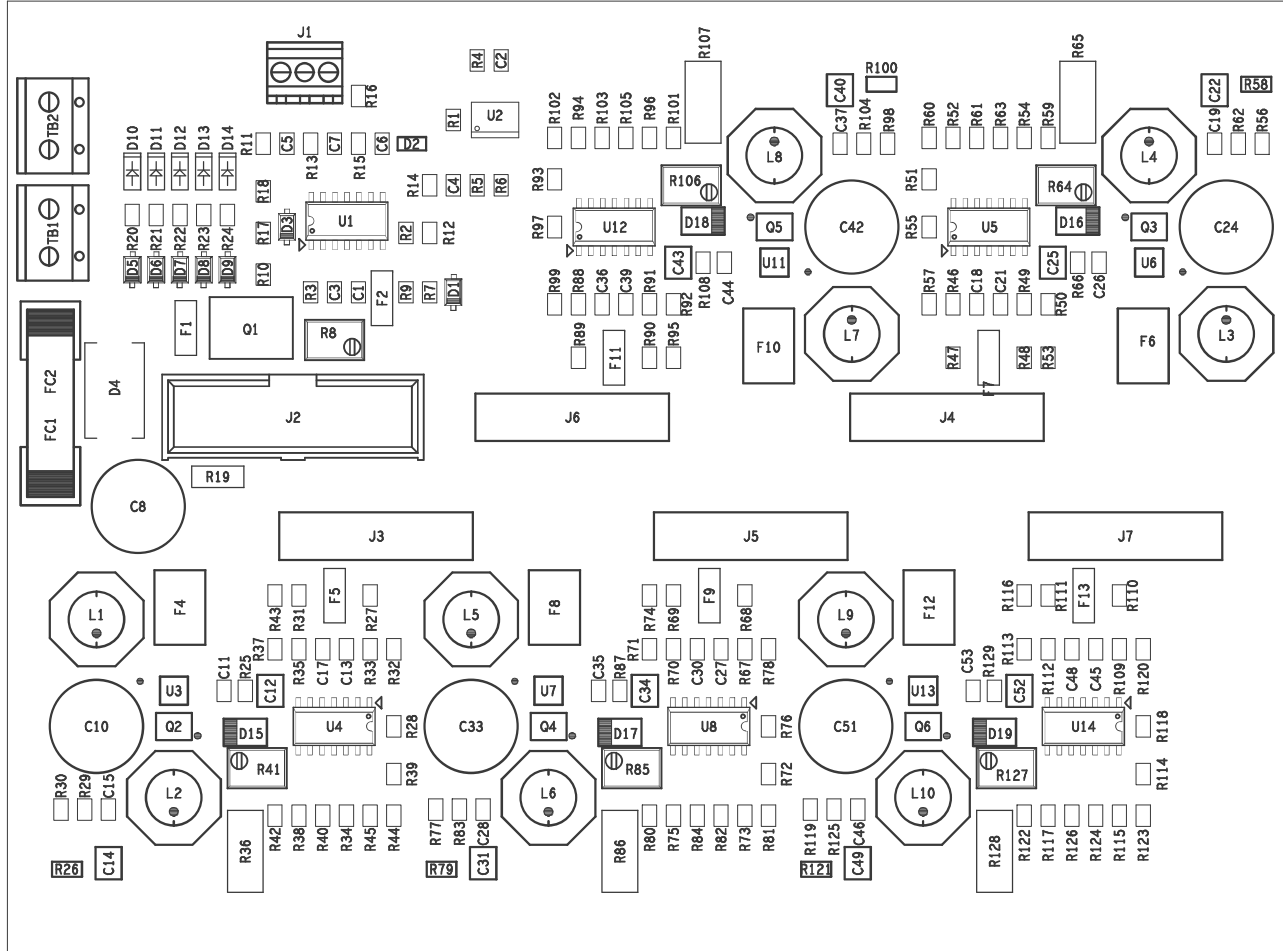
COMPONENT SIDE ASSEMBLY
